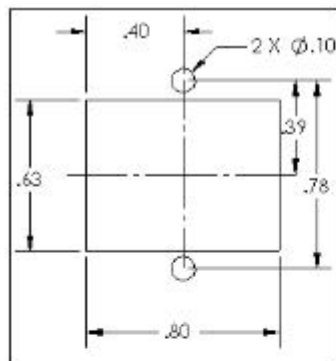
TRIM SWITCH CUT OUT PATTERN
