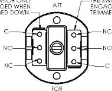
ELECTRICAL DIAGRAM
